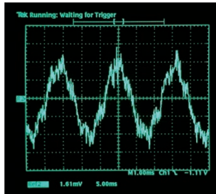
Brand "X" PWM scope trace (left) compared to smoother VVC+ scope trace (right).
