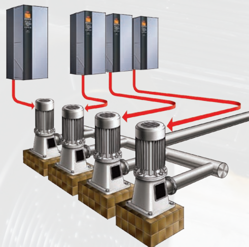
A typical VLT®AQUA Drive installation utilizing the Cascade Controller option via MODBUS in conjunction with three additional VLT®AQUA Drives to operate one to four pumps as demand requires.
