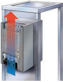
Through-panel mounting
