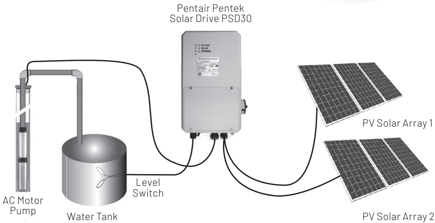
Figure 1: Solar Water Pumping System Diagram with Pentair Pentek Solar Drive PSD30
