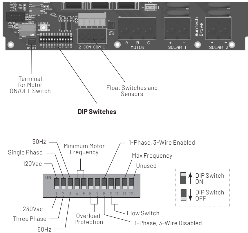
Figure 7: Pentair Pentek Solar Drive Printed Circuit Board Features Overview
