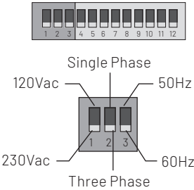
Figure 9: DIP Switches
