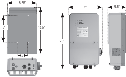
Figure 4: Dimensions du Pentair Pentek Solar Drive
