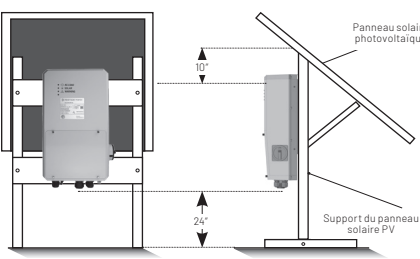
Figure 3: Montage du Pentair Pentek Solar Drive
