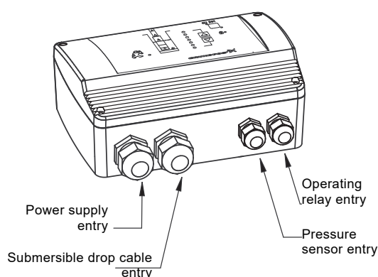
Fig. 19 Cable entries of CU 301
