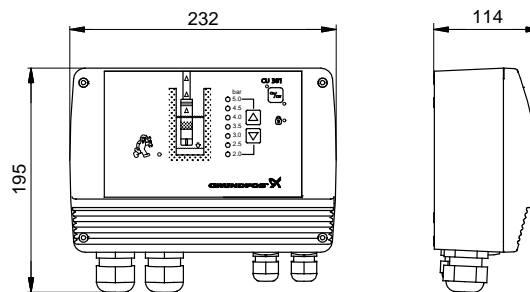
Fig. 20 Dimensional sketch of CU 301
