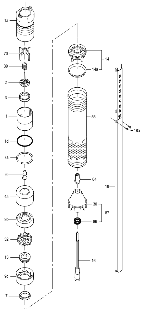
Fig. 30 Exploded view of pump and motor
