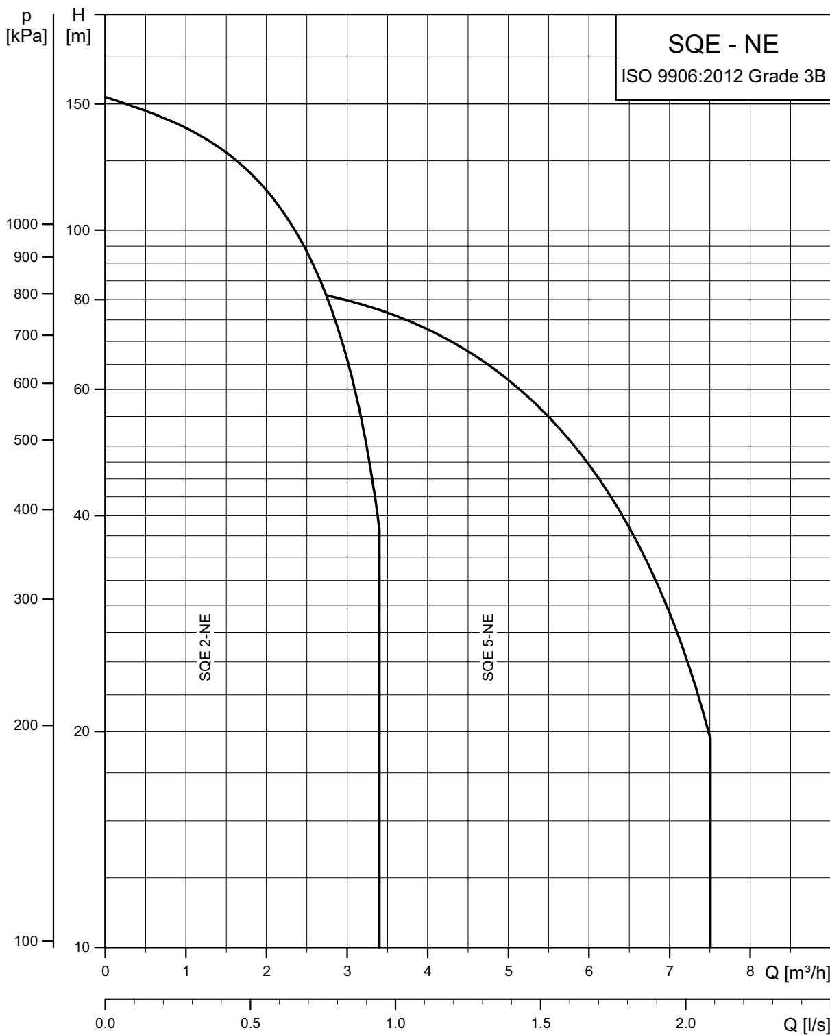
Fig. 2 Performance range, SQE-NE
