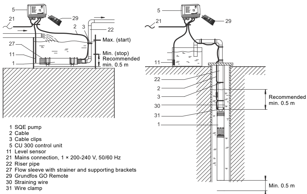
Fig. 13 Emptying or filling a tank
