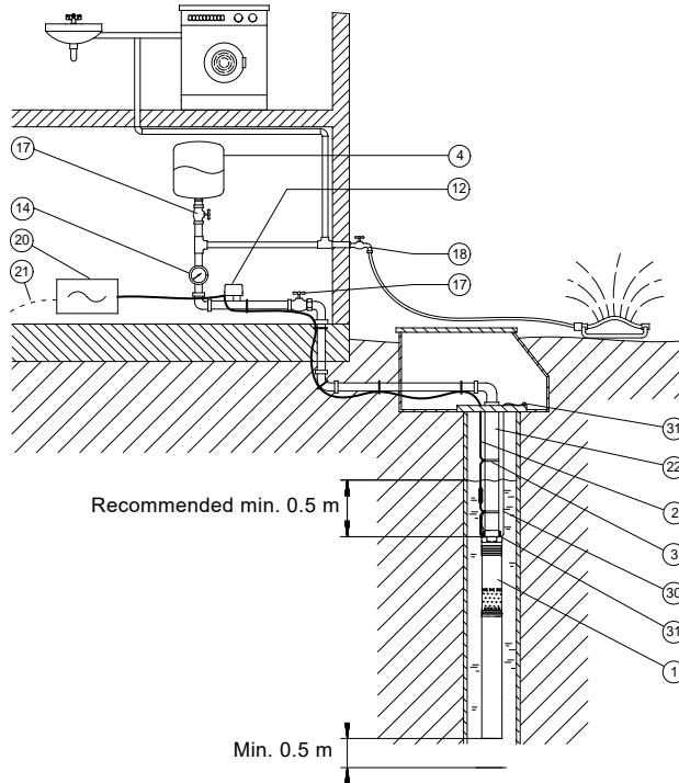
Fig. 8 Domestic water supply
